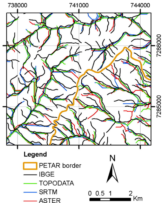
Fig. 4. Comparison between the three automatic extracted drainage networks and the official one.
